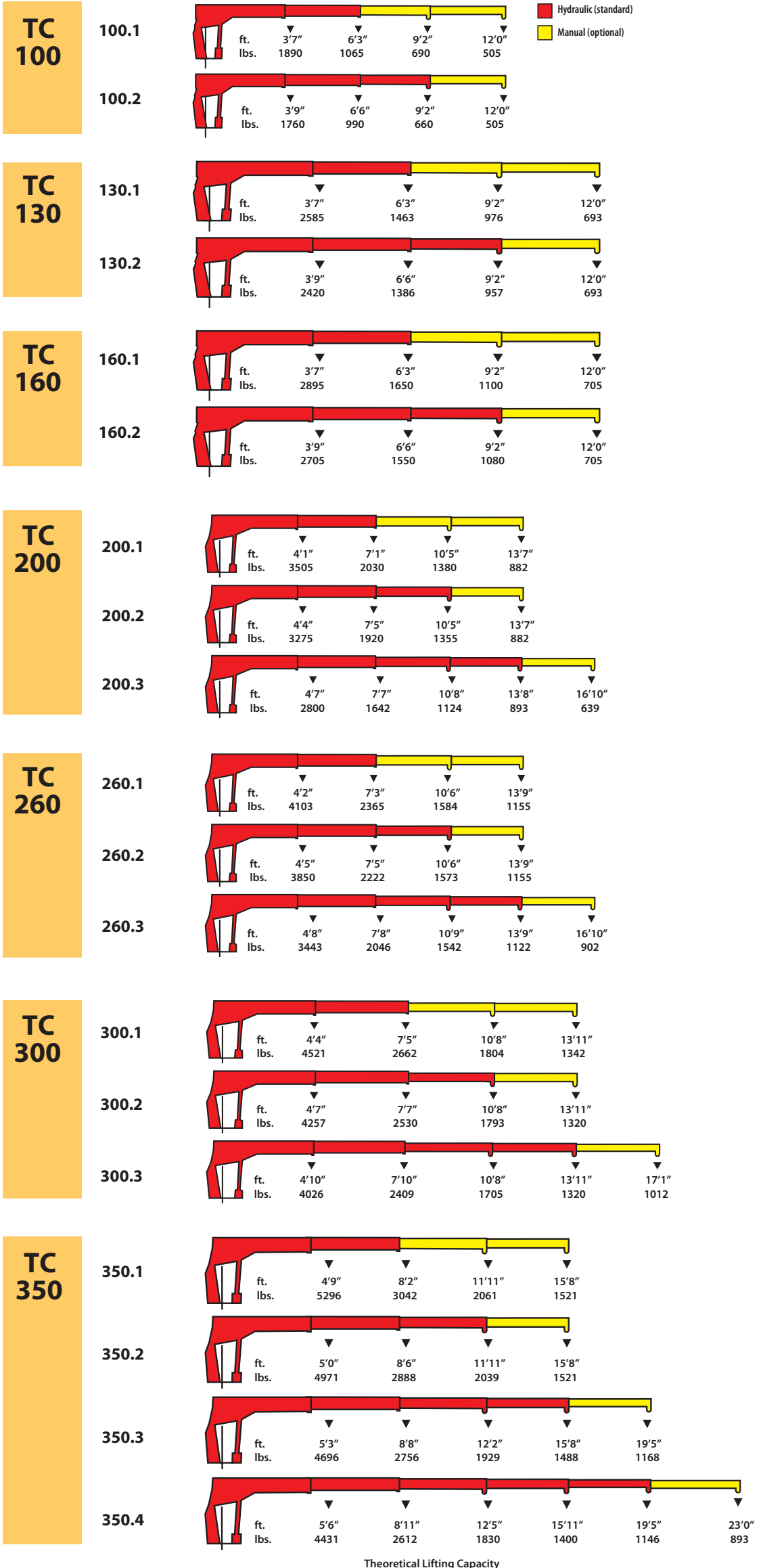
Theoretical Lifting Capacity
